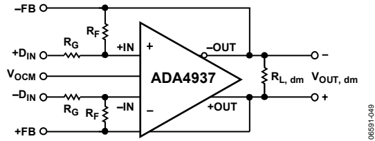
Figure 49. Circuit Definitions
